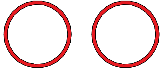
EL-0225 O-Ring,-023, Buna, 1-3/16x1-1/16x1/16 QTY 2
