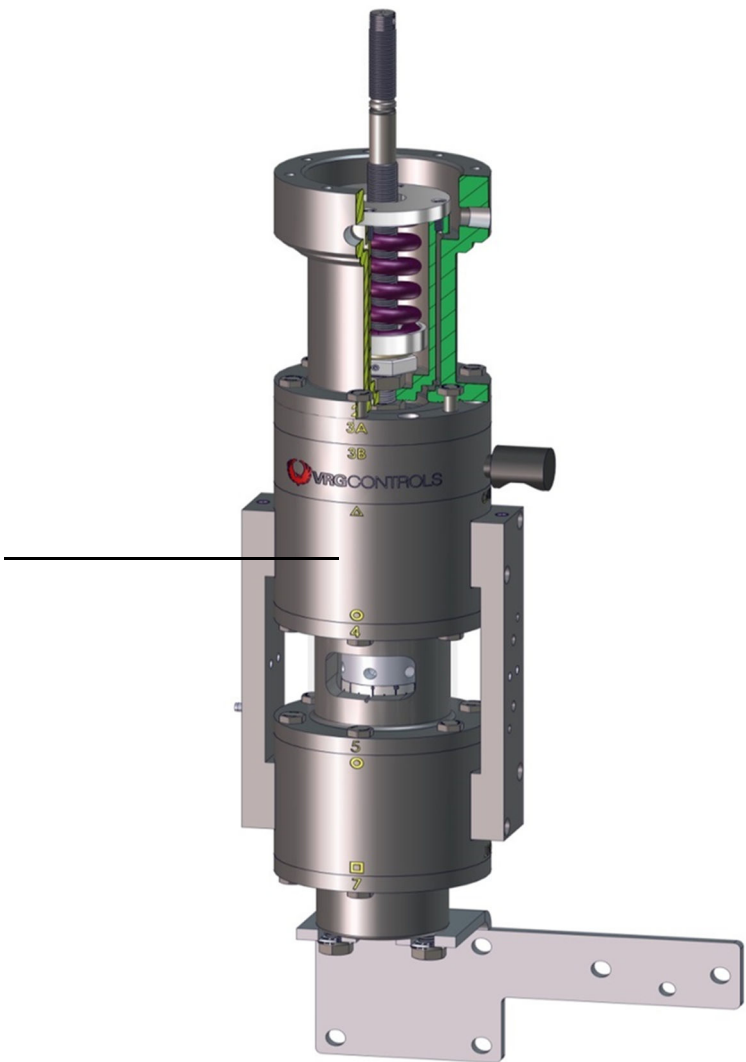
Pilot Blank Assembly with Setpoint Adjusting Screw Assembly Installed
