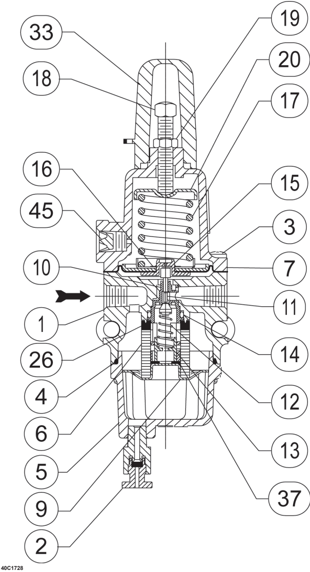
Figure 6. Type 67CFS or 67CFSR Assembly Drawing
