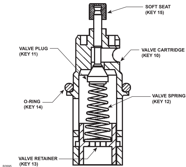
Figure 12. Valve Cartridge Assembly
