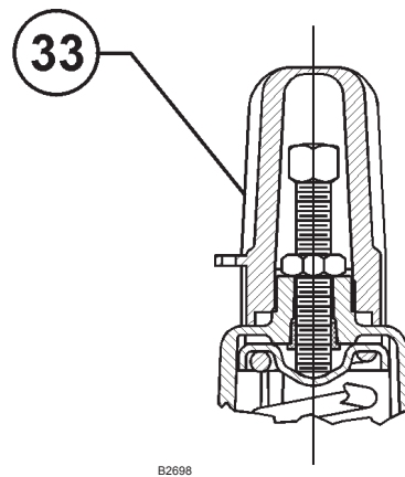
Figure 11. Optional Closing Cap [Only Available with the 1/4-inch (6,35 mm) Spring Case Vent]
