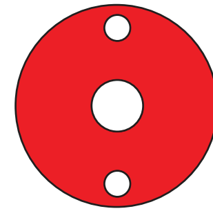
PD-0312 Piston with 1/2 DIA Molded Seat; for 1/4 Nozzle STD-1.5 QTY 1
