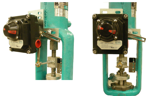
CVS Linear Actuator with CVS 500 Limit Switch
