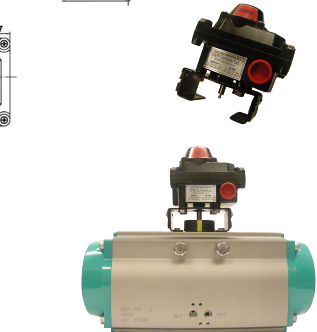
CVS 140SR Rack and Pinion Actuator with CVS 500 Limit Switch
