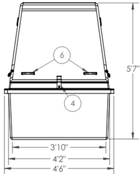
FRONT VIEW (CLOSED)
