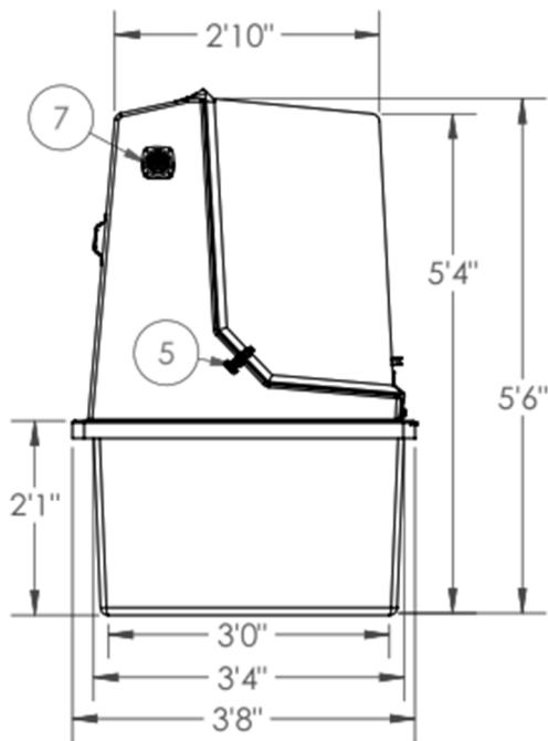
LEFT SIDE VIEW (CLOSED)
