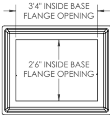
BOTTOM VIEW (CLOSED)
