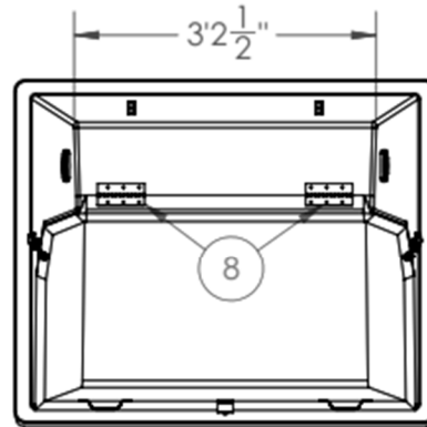
TOP VIEW (CLOSED)
